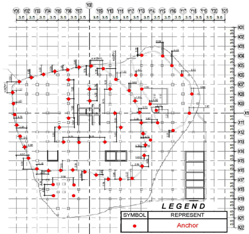
Fig. 10. Anchors Layout
