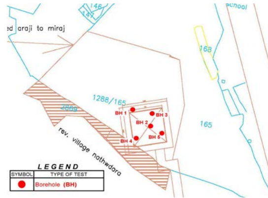
Fig. 4. Layout plan showing borehole locations
