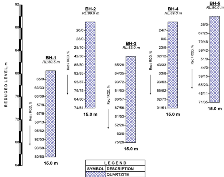
Fig. 7. Typical boreholes profile
